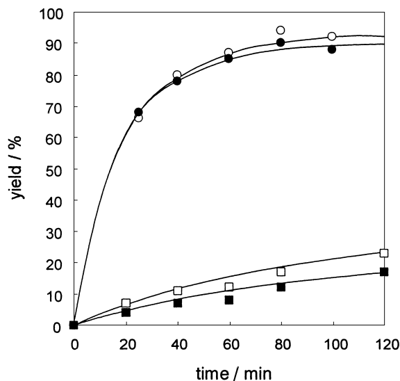
Fig. 1. Time-courses of thermolysis of 1b at 80 °C in water. Ethylene (○) and ethane (●) evolved in the absence of TPPTS ([ 1b ] = 7.2 mmol/L); ethylene (□) and ethane (■) evolved in the presence of TPPTS ([ 1b ] = 7.0 mmol/L, [TPPTS] = 34.8 mmol/L).
